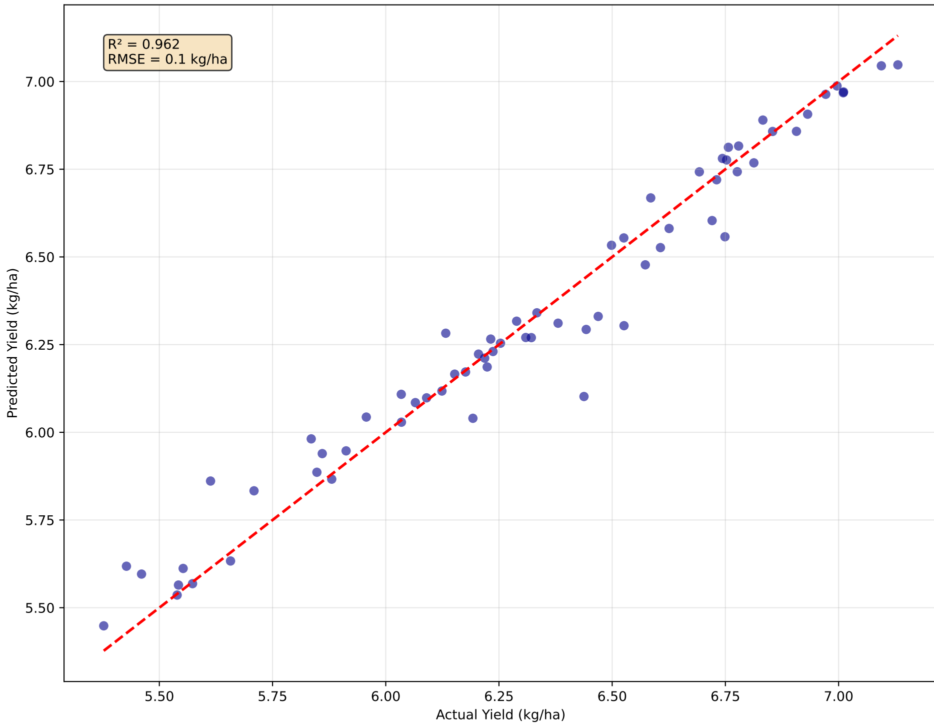
Predicted vs Actual Yield ( R^2 = 0.962 )
