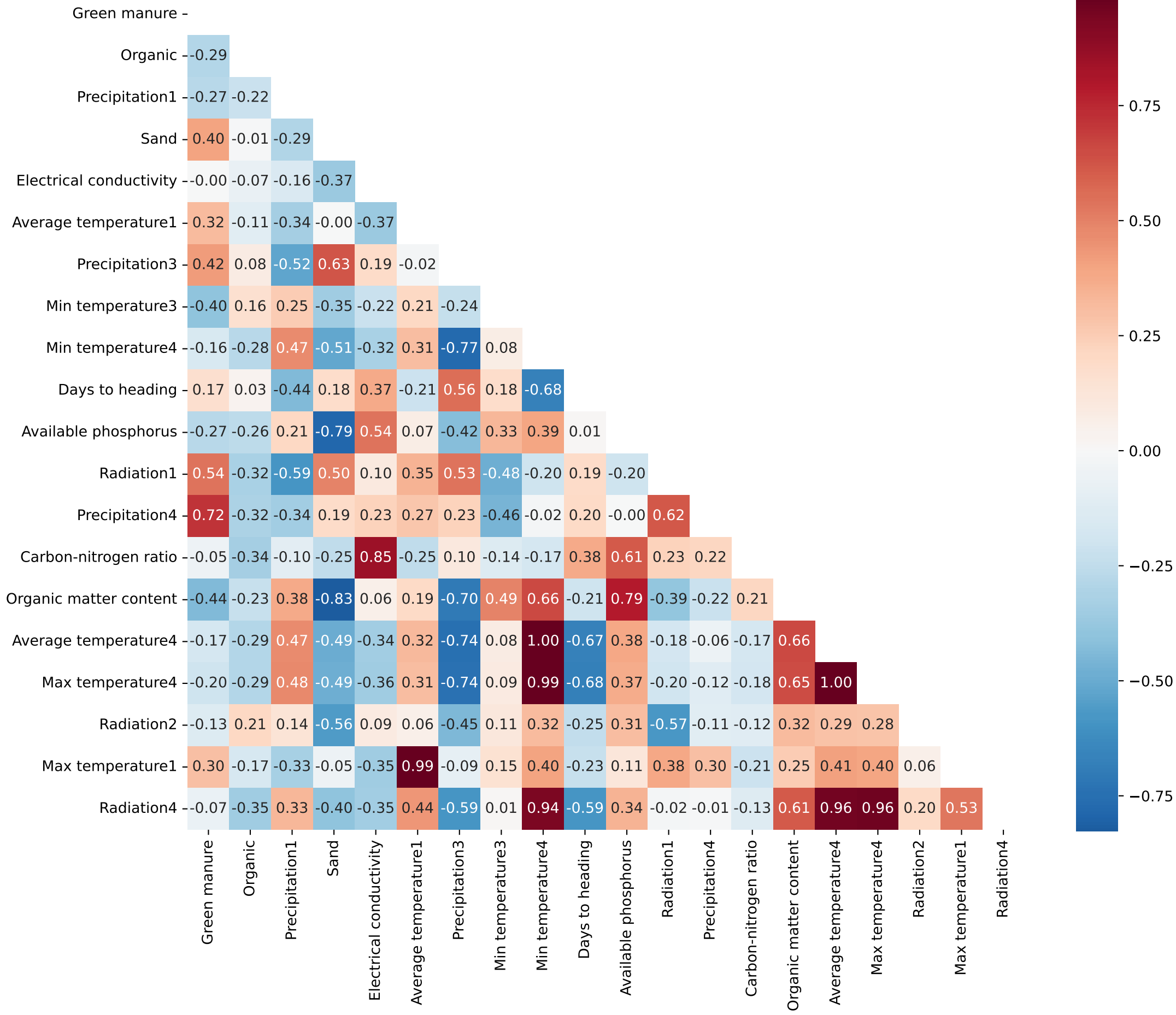
Correlation Matrix - Top 20 Yield-Predictive Variables
