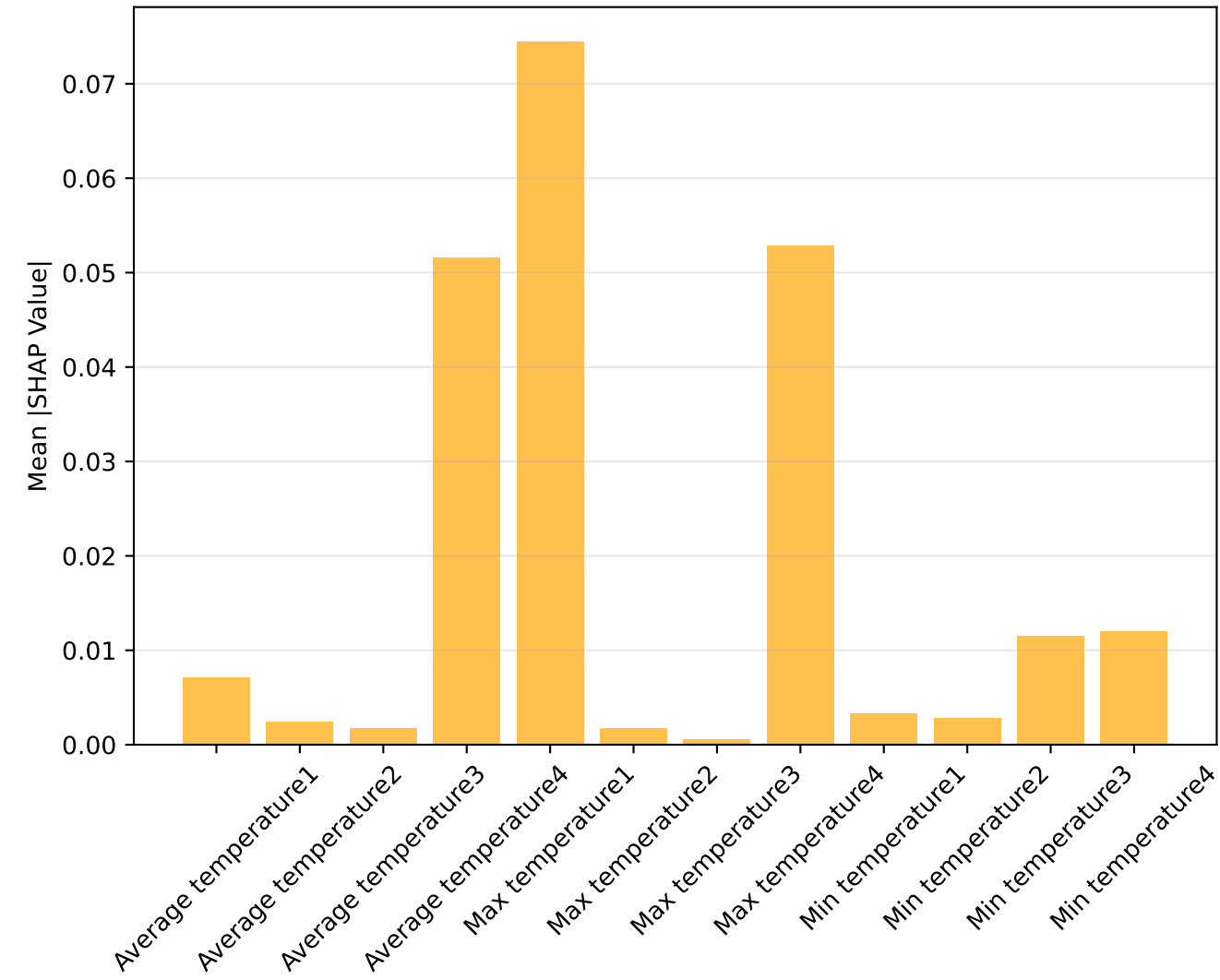
Temperature Variable Importance by Growth Stage
